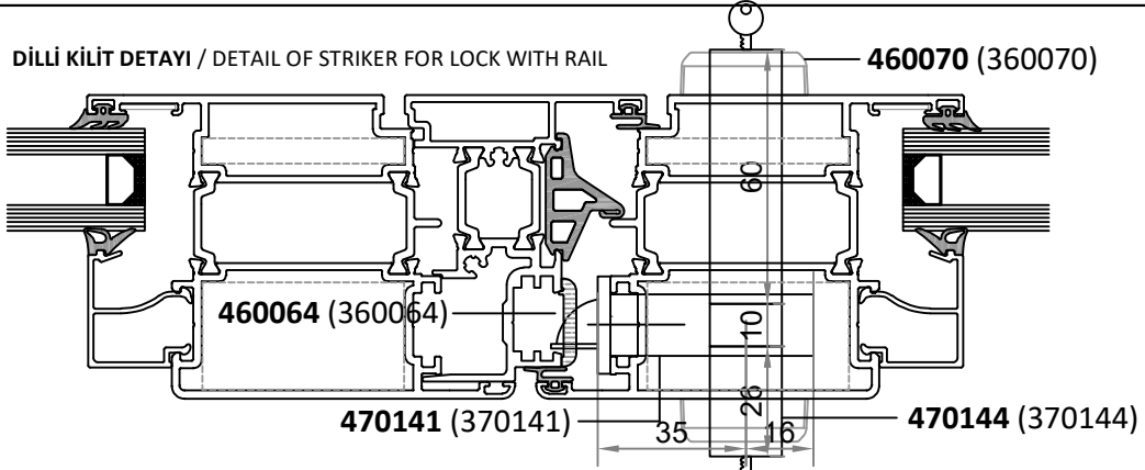
MAKARALI KİLİT DETAYI / DETAIL OF STRIKER FOR LOCK WITH ROLLER
