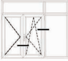
PVC AKSESUARLI PENCERE DETAYLARI WINDOW DETAILS WITH PVC ACCESSORY
