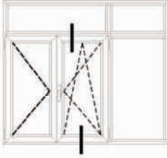
PVC AKSESUARLI PENCERE DETAYLARI WINDOW DETAILS WITH PVC ACCESSORY
