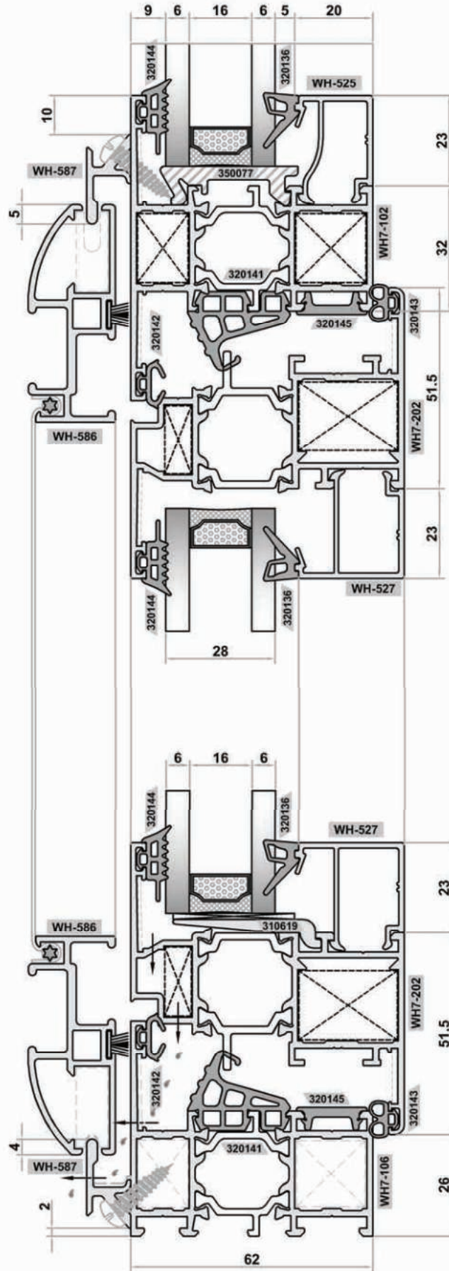
PENCEREYE ENTEGRE KAYAR SİNEKLİK DETAYLARI WINDOW INTEGRATED SLIDER INSECT SCREEN DETAILS
