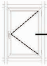
KAPAKLI CEPHE İÇİ DOĞRAMA DETAYI CASEMENT DETAIL IN CAPPED CURTAIN WALL
