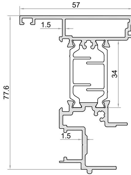
W8-503 AĞIRLIK / WEIGHT (KG/M.) 1,514 (PVC) 1,491 (POL.)
