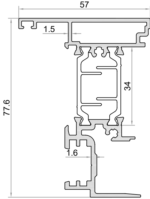
W8-502 AĞIRLIK / WEIGHT (KG/M.) 1,549 (PVC) 1,527 (POL.)
