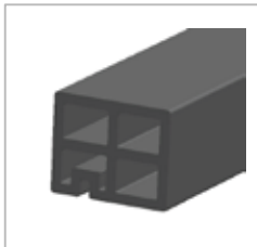
W65 GİZLİ KANAT YALITIM SÜNGERİ INSULATION FOAM FOR W65 HIDDEN SASH 490083 (390083)
