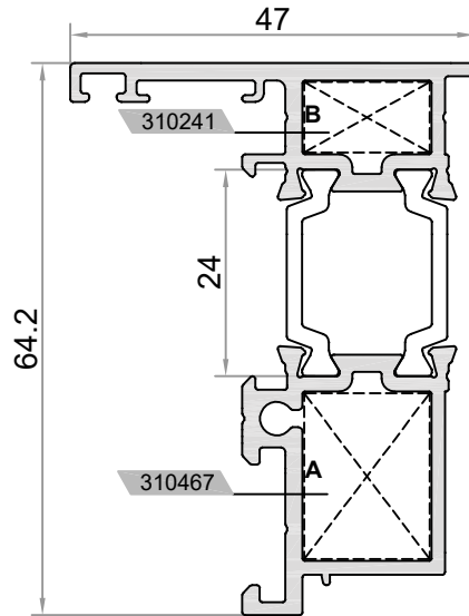
W6-510 AĞIRLIK / WEIGHT (KG/M.) 1,262 (PVC) 1,247 (POL.) VİDALI KÖŞE TAKOZLARI SCREW CORNER CLEATS 310466 (A) 310178 (B)
