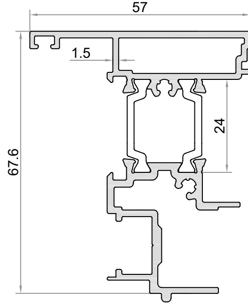
W6-509 AĞIRLIK / WEIGHT (KG/M.) 1,417 (PVC) 1,402 (POL.)
