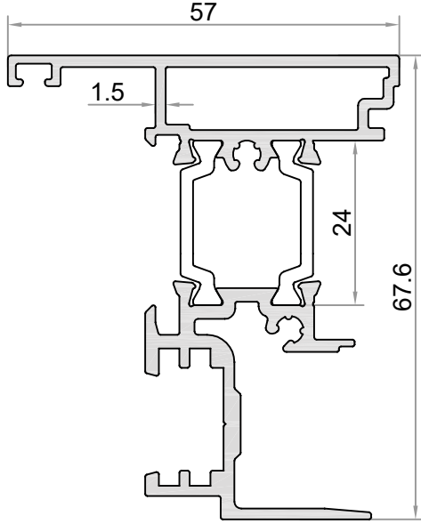
W6-508 AĞIRLIK / WEIGHT (KG/M.) 1,453 (PVC) 1,438 (POL.)
