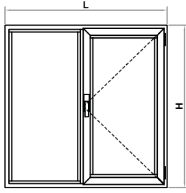
TEK TARAFI SABİTLİ TEK AÇILIM PENCERE ONE SIDE FIXED SIDE HUNG OPENING WINDOW
