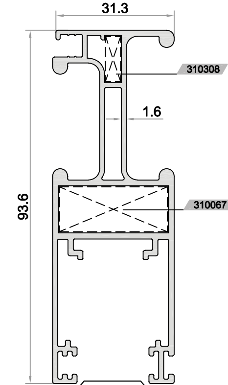
S3-514 AĞIRLIK / WEIGHT (KG/M.) 1,420
