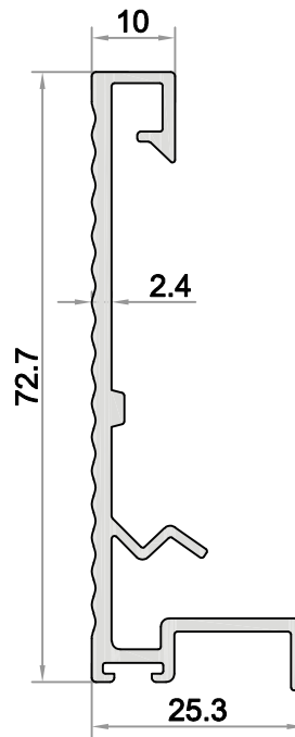
S3-516 AĞIRLIK / WEIGHT (KG/M.) 0,721
